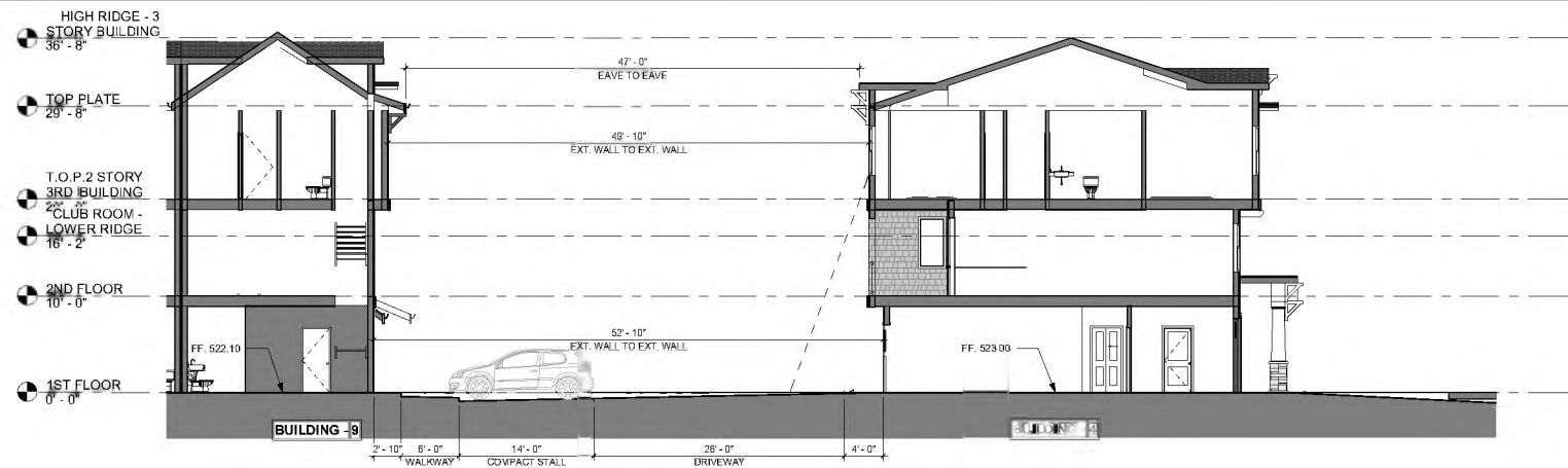
1 TYPICAL SECTION NORTH TO SOUTH - BLDG 4 & 9 1/8" = 1'-0"
