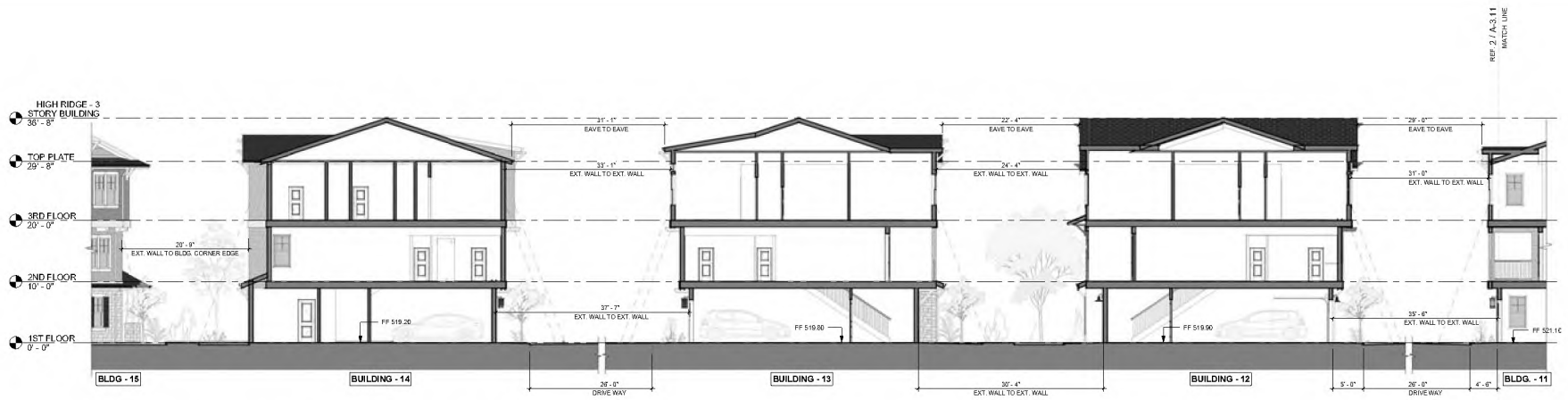
① TYPICAL SITE SECTION WEST TO EAST - BLDG. 11, 12, 13, 14, 15 1/8" = 1'-0"
